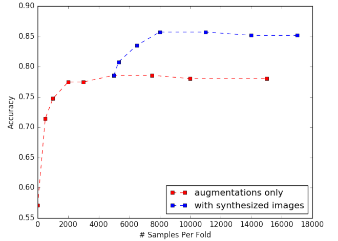
Fig. 3: Accuracy results for liver lesion classification with the increase of training set size. The red line shows the effect of adding classic data augmentation and the blue line shows the effect of adding synthetic data augmentation.
